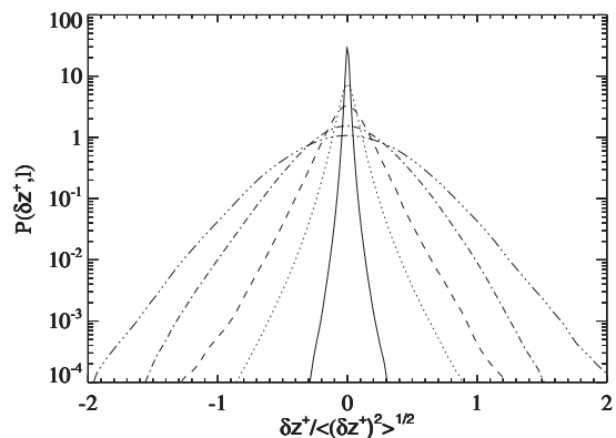
FIG. 5. The PDFs of Elsässer field fluctuations \delta z^+ for the same five different scales as in Fig. 1.
