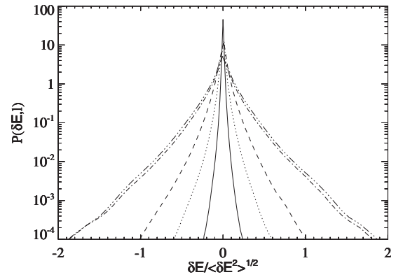
FIG. 1. The PDFs of total energy fluctuations \delta E on five different scales \ell = \pi/n with n=511 (solid), n=130 (dotted), n=46 (dashed), n=4 (dot-dashed), and n=1 (three-dot-dashed).
