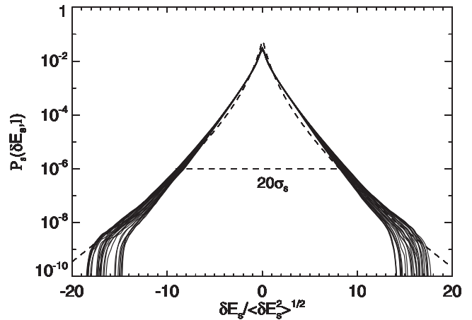
FIG. 4. Rescaled PDFs of total energy fluctuations in the inertial range of the Navier-Stokes case (c). The gamma law 10^{-3}\exp(-|\delta E|/0.4)|\delta E|^{-3.4} is represented by the dashed curve.
