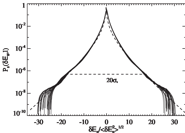
FIG. 3. Rescaled PDFs of total energy fluctuations in the inertial range of the isotropic case (a). The gamma law 10^{-3}\exp(-|\delta E|/0.35)|\delta E|^{-3.1} is represented by the dashed curve.
